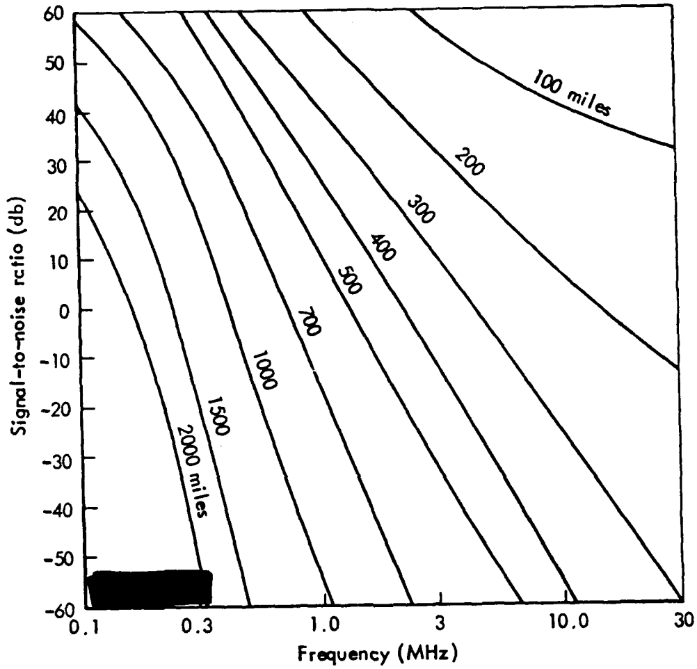
Fig. 5-4 Signal to-noise ratio vs frequency (ground wave transmission over land)
